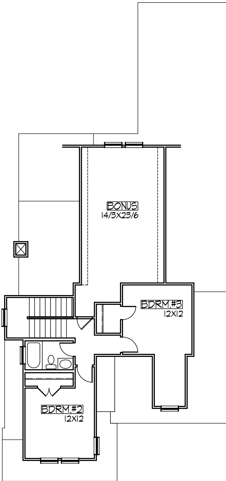
SECOND FLR. PLAN
